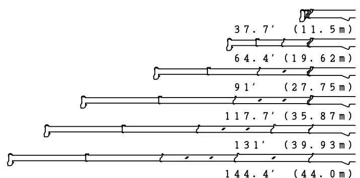
Boom Length in Feet (Telescoping Mode II)
