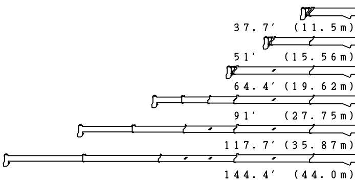
Boom Length in Feet (Telescoping Mode I)
