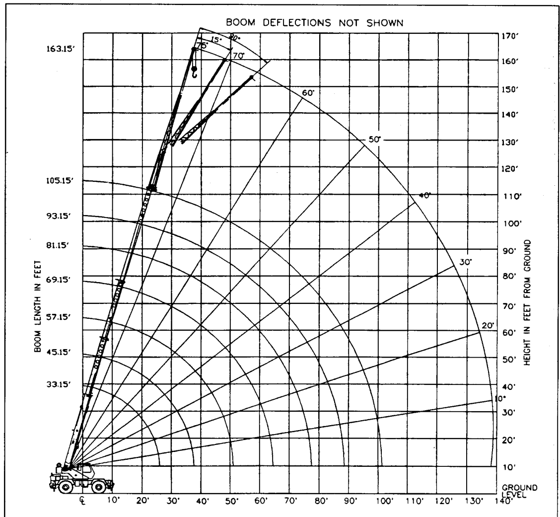
Range Diagram (33' - 105' boom)
