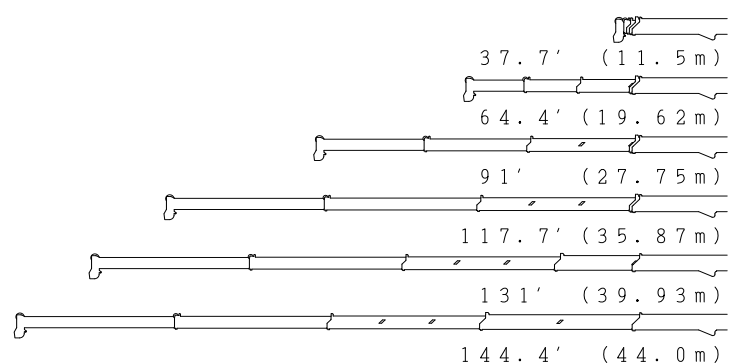
Boom Length in Feet (Telescoping Mode II)
