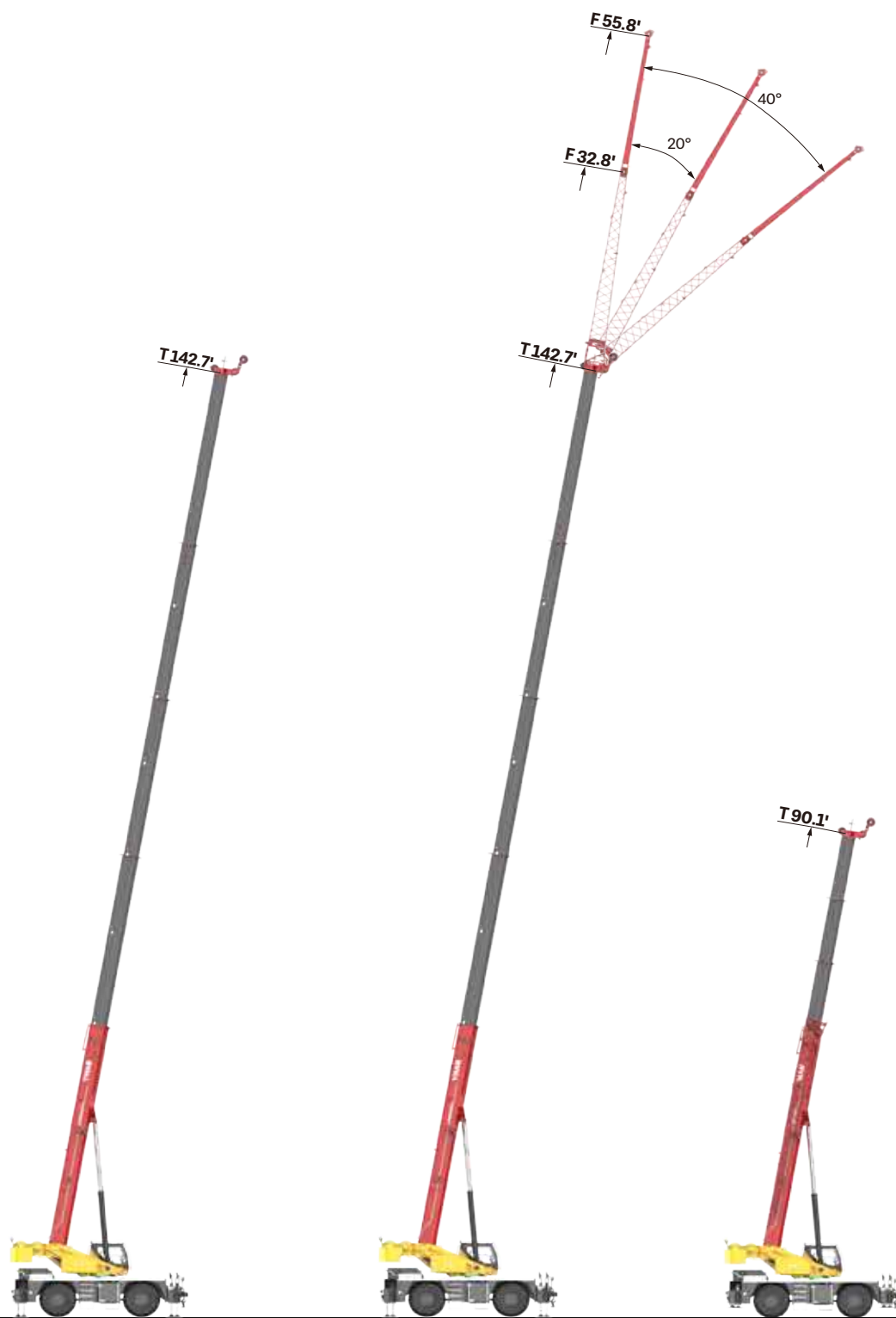
Main Boom On Outriggers
