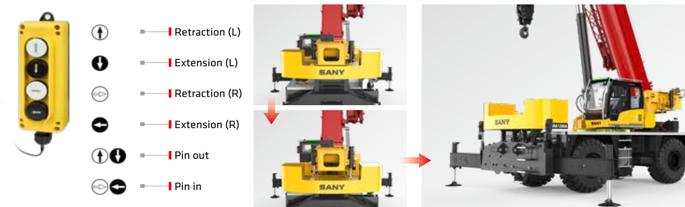
Remote controller
