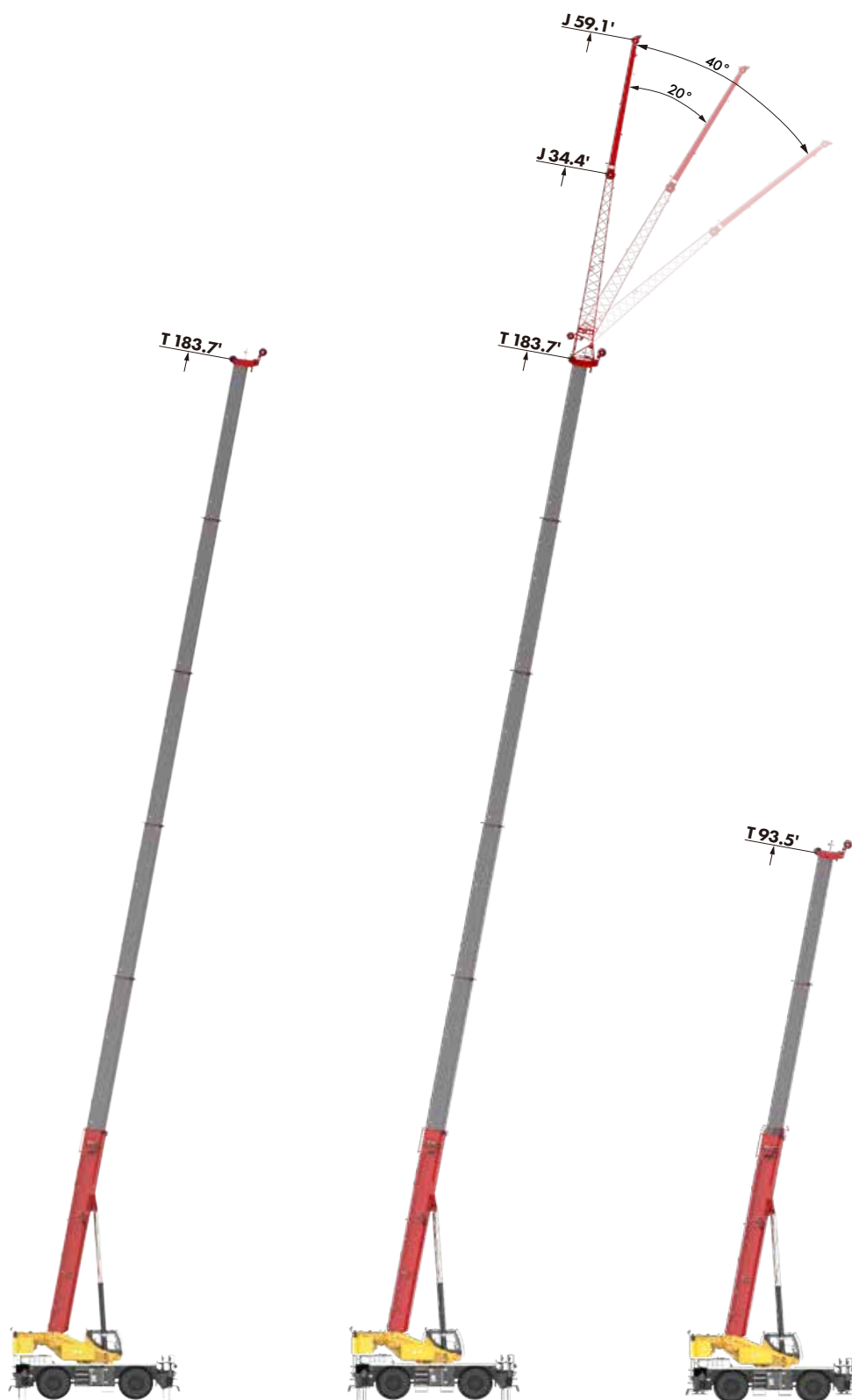
Main Boom On Outriggers
