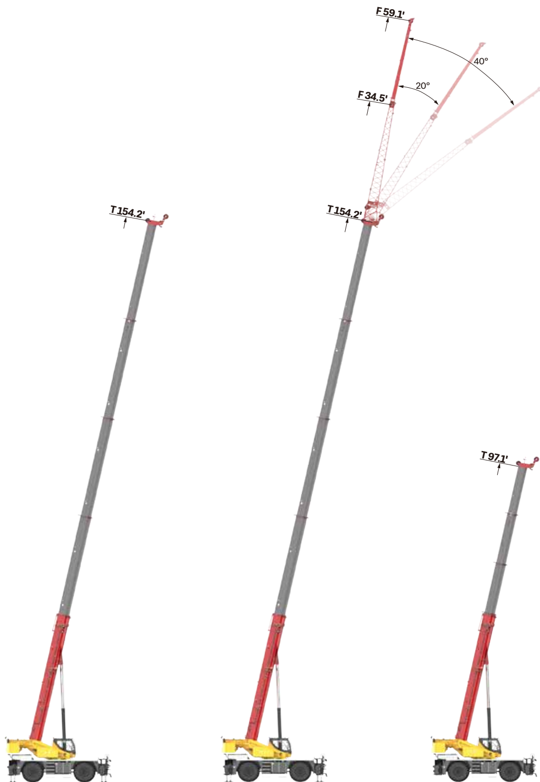
Main Boom On Outriggers
